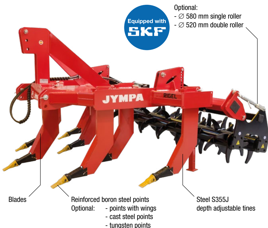
Model RIGEL-7-2V-440 with Ø 520 mm double roller and cast steel points
