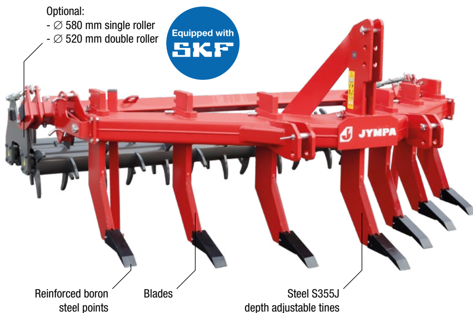
Model ANTARES-7 with Ø 520 mm double roller
