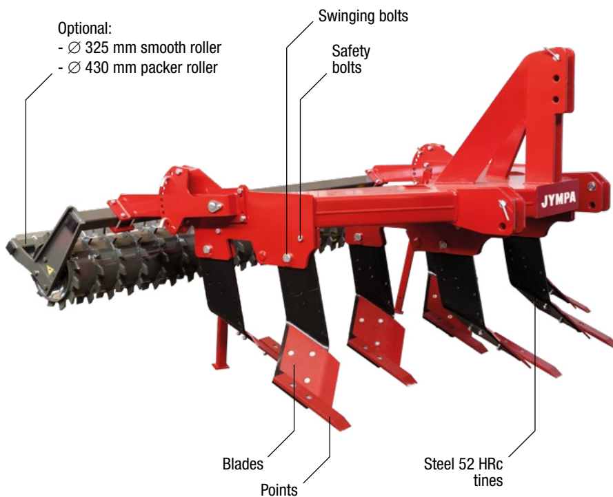
Model MINTAKA-4 with Ø 430 mm packer roller
