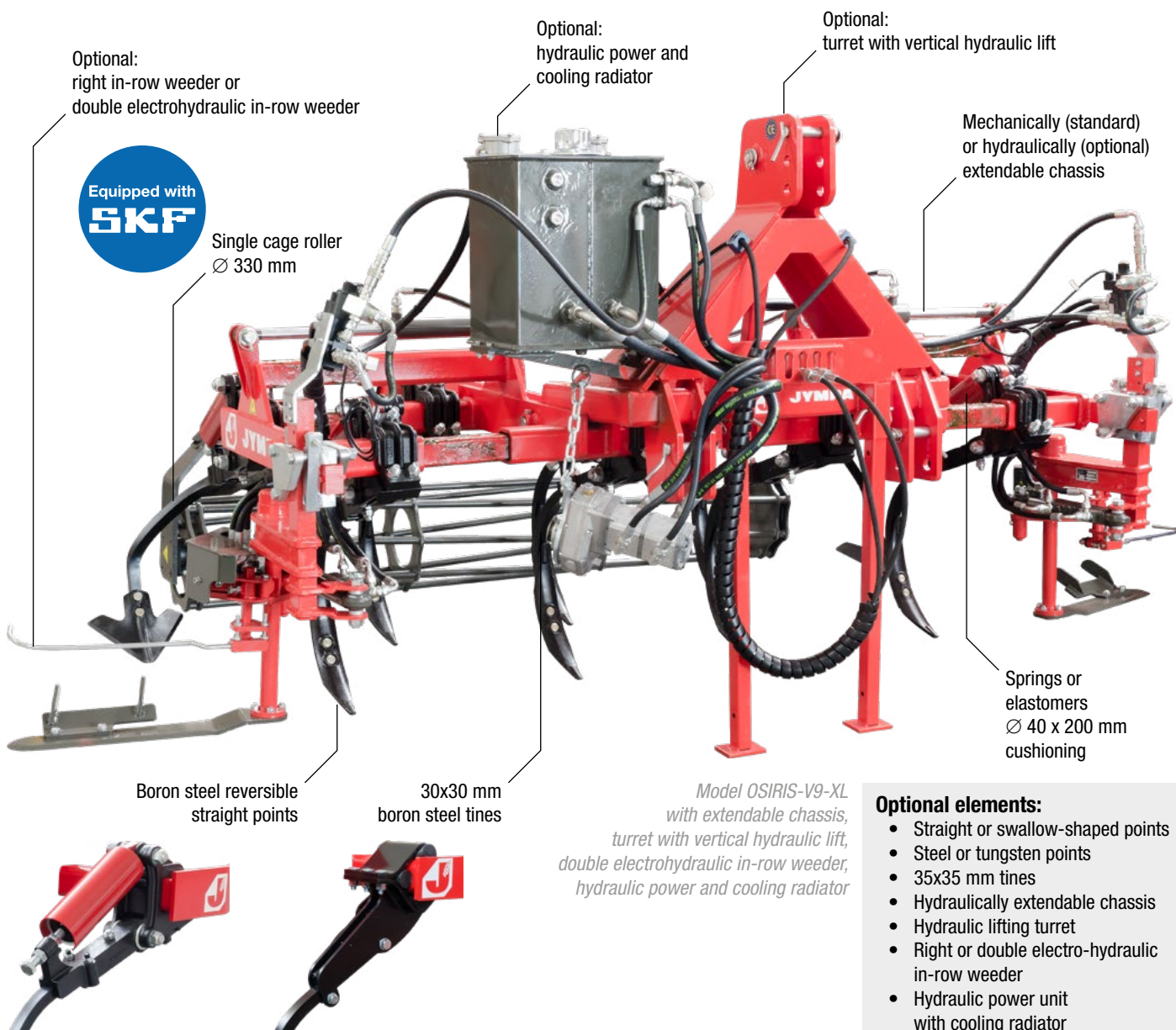
Tines with spring or elastomer cushioning
