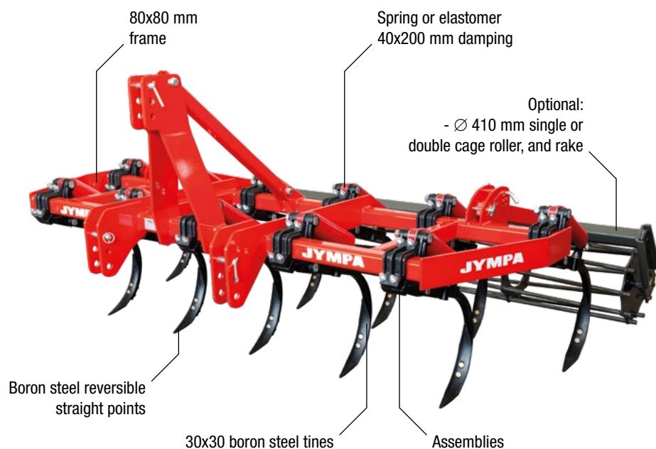
Model OSIRIS-11-2F with Ø 410 mm single cage roller
