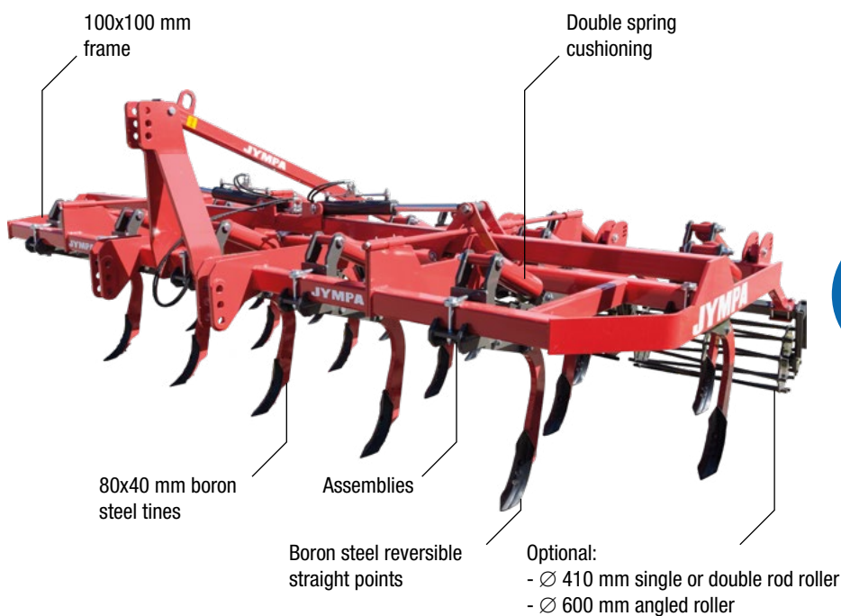
Model NIKKAL-17-3F-PL with Ø 410 mm single cage roller
