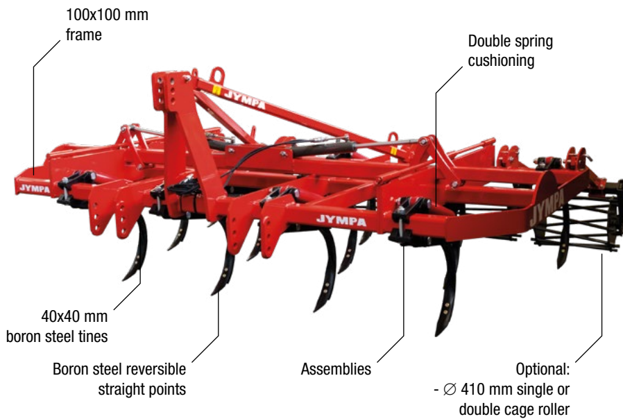
Model DAGON-13-3F-PL with Ø 410 mm single cage roller
