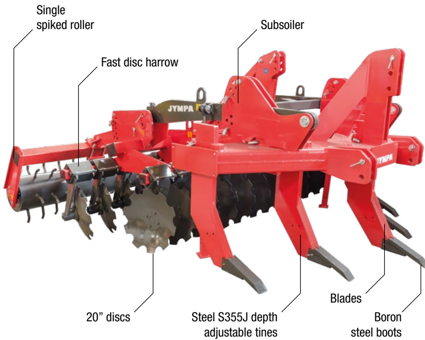
Model TANDEM-3000
