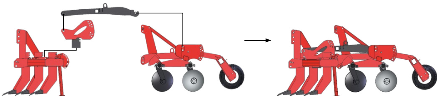
Subsoiler + Roller
